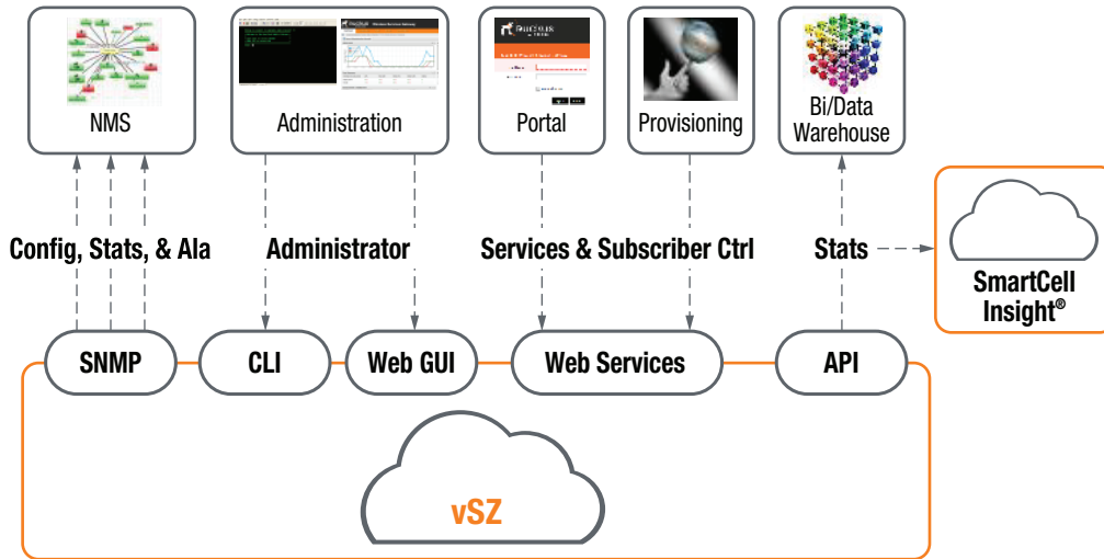
Figure 2: The built-in EMS in the vSZ-H provides user-friendly full-fledged FCAPS support and can be easily integrated with existing OSS/BSS systems.
