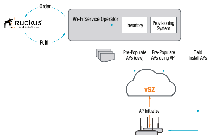
Figure 3: Automatic Access Point Configuration is the process by which APs installed in the field can have their configuration automatically downloaded to them via the vSZ-H.
